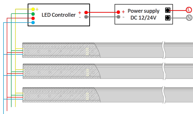
Solderless wiring (20mm & 180mm)
